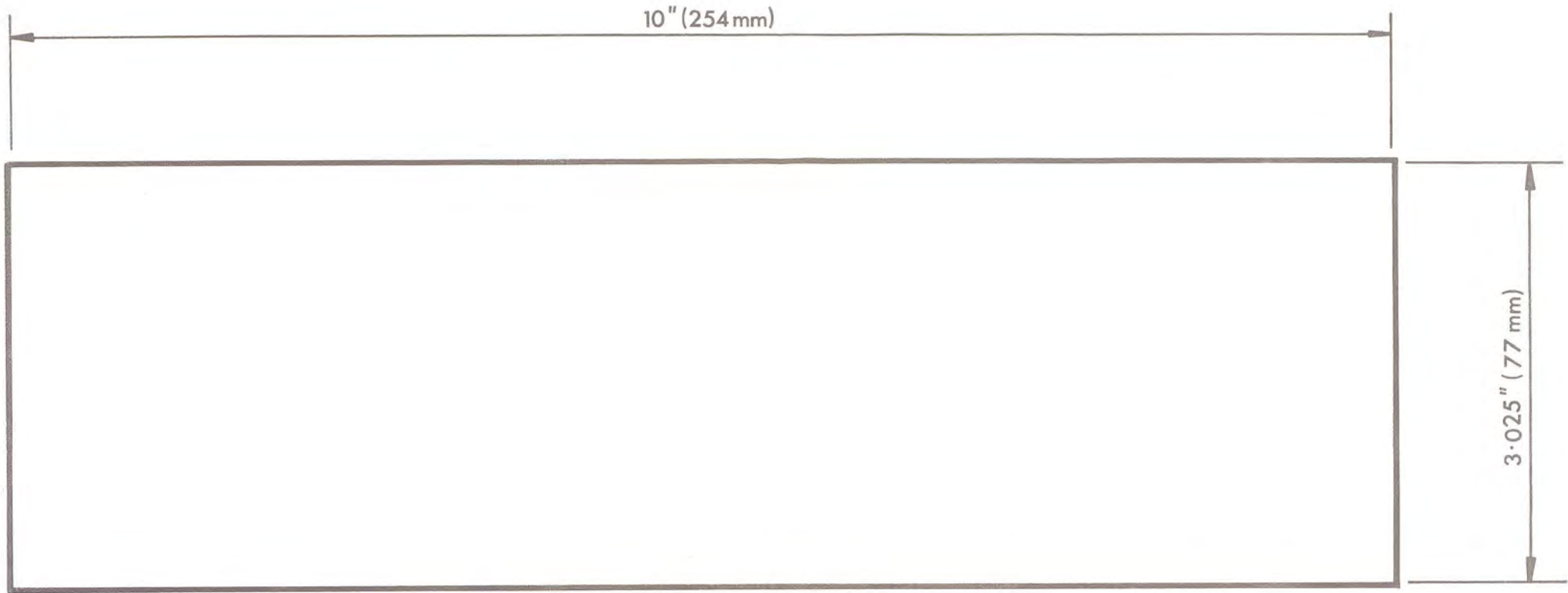
CUTOUT TEMPLATE FOR QUAD CONTROL UNIT & TUNER
