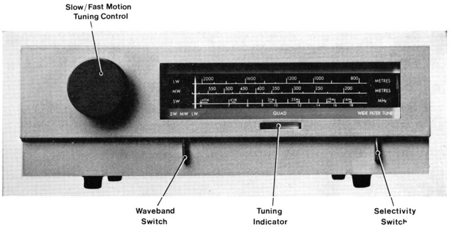
Fig. 8 Front panel view
