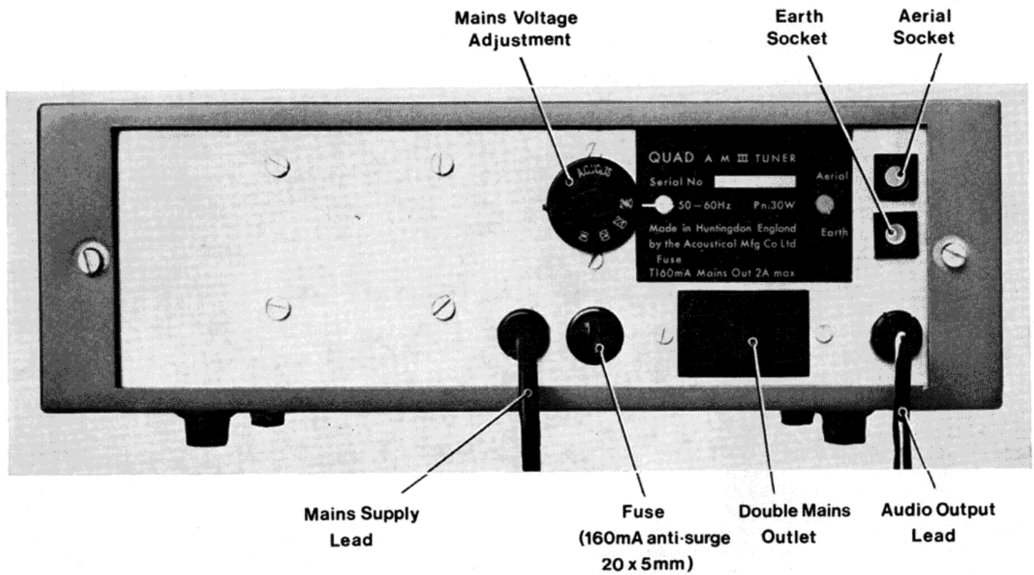
Fig. 1 Rear panel view
