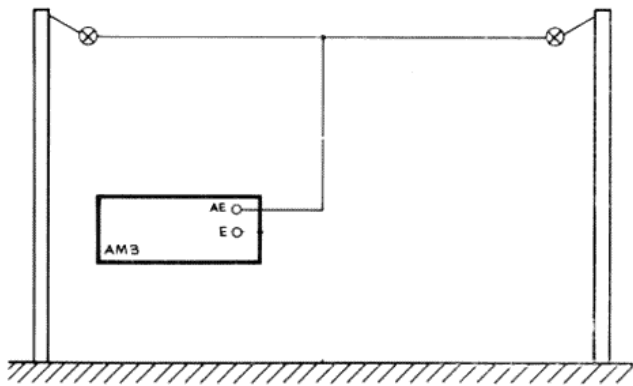
Fig. 4 T aerial
