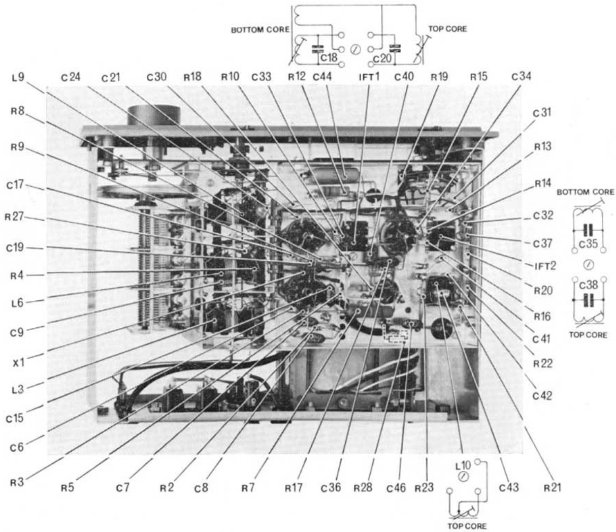
Fig. 10 Under chassis view
