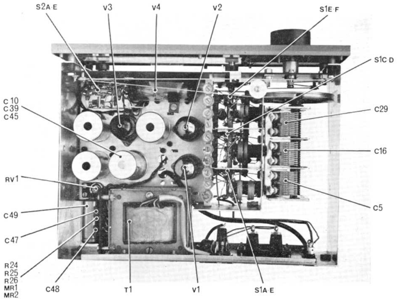
Fig. 9 Above chassis view
