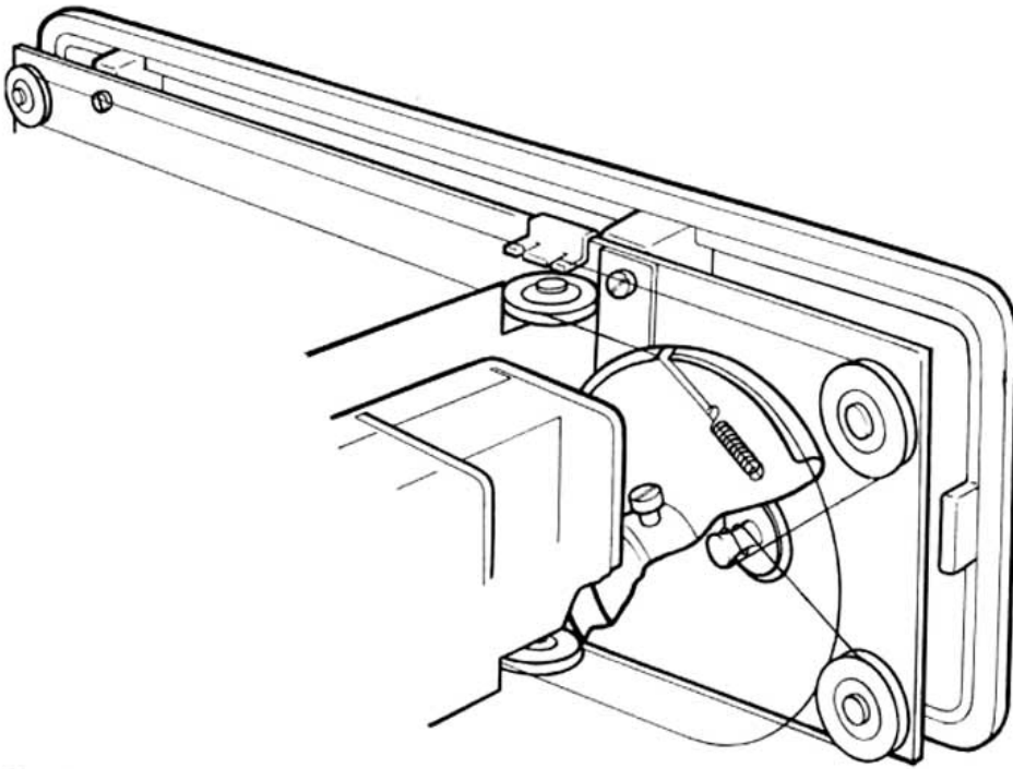
Fig. 13 Replacing the drive cord 18
