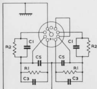
SINGLE LETTER ADAPTOR
